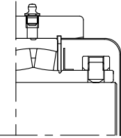
End cover (suffix Y, 3 7/16" shaft and up)
