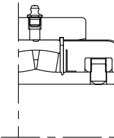
End cover (suffix Y, 3 7/16" shaft and up)
