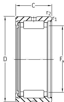
Series RNA 49 RS
