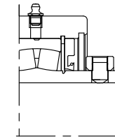
Garter spring seal (suffix - 3)
