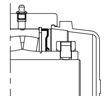
End cover (suffix Y, 1 3/16" to 3" shaft)
