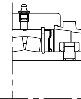
End cover (suffix Y, 1 3/16" to 3" shaft)
