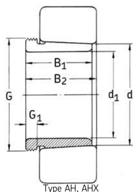
Type AH, AHX
