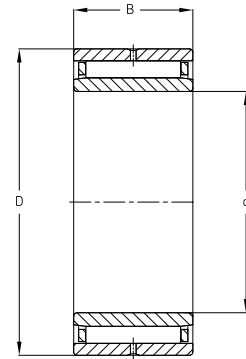
Series NKI
