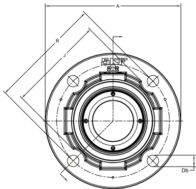
FYR 1 3 / 16 N thru 1 1 / 2 N have three mounting holes at 120°
