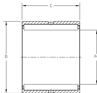
Series NKS
