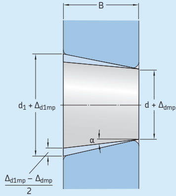
Largest theoretical diameter d_1 d_1 = d + \frac{1}{12} B
