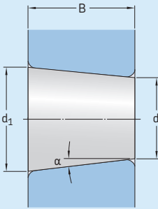
Half angle of taper 1:12 \alpha = 2^\circ 23' 9,4''
