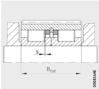
Axial clearance s
