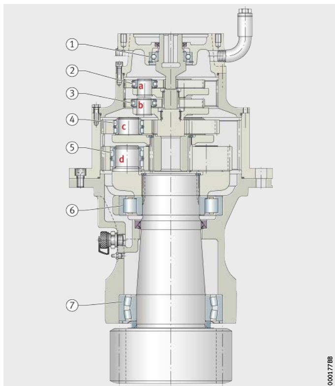
Figure 2 Bearing positions in pitch and yaw gearbox
