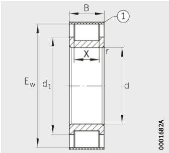
RSL1823...-A ① Mounting sleeve
