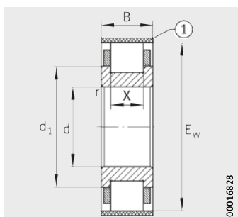
RN2...E-MPBX ① Mounting sleeve
