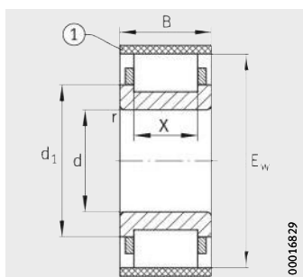
RN22...-E-MPBX (-EX-MPBX)
