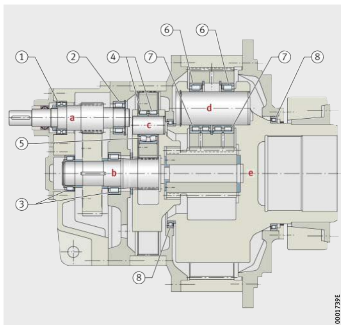
Figure 2 Bearing positions in the planetary gearbox
