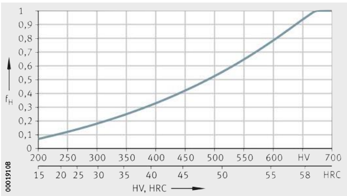
Figure 3 Dynamic hardness factor f_H
