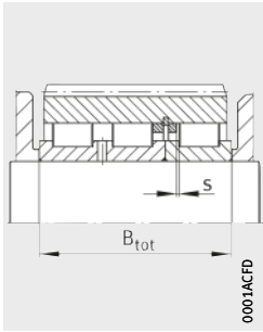
RSL1850, RSL1830 Axial clearance s 1)
