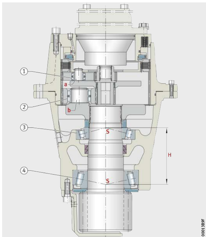
Figure 2 Bearing positions in the slewing gear drive
